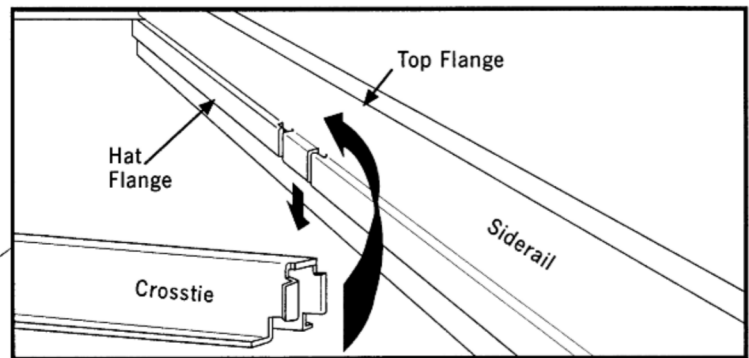
Detail 2
